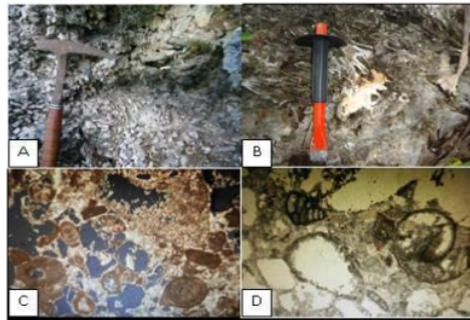
Figure 5. Field view of branching coral (A & B) cropping out at the southern part of Pleistocene reef (just right the top of siliciclastics rock). Microphotograph of matrixes of the Reef Front Facies consists of foraminifera rich grainstone (C), and coral fragments bioclastic grainstone (D).
