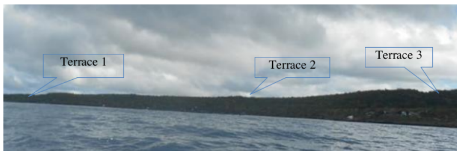
Figure 4. Morphology of west coast showing 3 sub terraces of Pleistocene reef.
