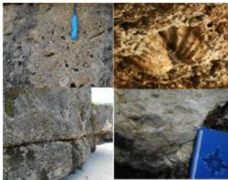
Figure 6 Outcrop of reef core facies showing rhodolite channel-like deposits at lower bed (A), and in some places, Tridacna sp. are present (B) at the upper part of the reef core facies. (C) and abundant coral fragments (D).
