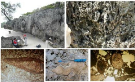
Figure 7 Outcrop of back reef facies along the west coast (A) with abundant branching coral (B) and small amount of red algae in thin section (C) rare Tridacna sp (D) and Calcarina spin thin section (E).
